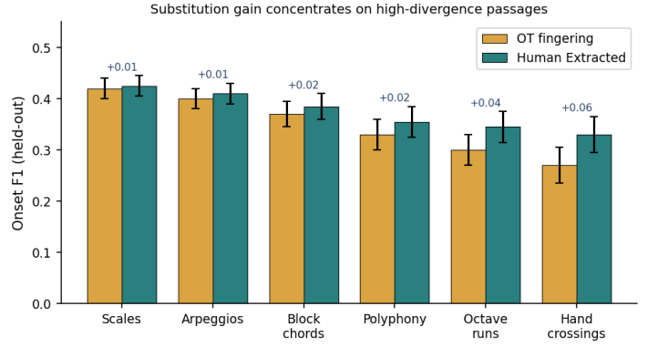
Figure 16: Held-out Onset F1 by passage type, OT vs. extracted fingering under PLR. Gain concentrates where OT and humans most disagree.
