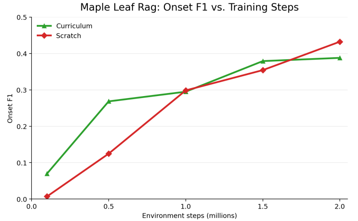
Figure 11: Onset F1 during Maple Leaf Rag training.
