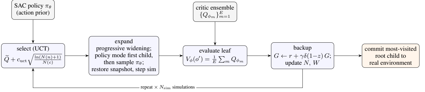
Figure 5: Depth-limited MCTS-style planner for one control step (Section 4.3). The agent plans over the exact simulator: it runs N_{\text{sim}} simulations that descend by UCT, expand under progressive widening (the policy mode is the first child, later children sampled from \pi_\theta ), restore the selected node’s full simulator snapshot and step it once, value a nonterminal leaf by the critic-ensemble mean (terminal leaves take value zero; a depth- D leaf uses the critic without further expansion), and back the return up the selected path. After N_{\text{sim}} simulations the agent commits the most-visited root child to the real environment and replans at the next control step. The policy and critic are the only learned components; the simulator supplies an exact model, so planning adds no new dynamics knowledge.
