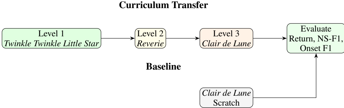
Figure 8: Hand-designed curriculum for Clair de Lune . Policies are trained sequentially on increasingly difficult repertoire before transfer to the target piece. Each stage receives 2M environment steps.
