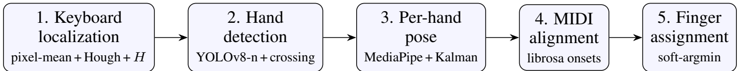
Figure 14: Five-stage video-to-fingering pipeline.
